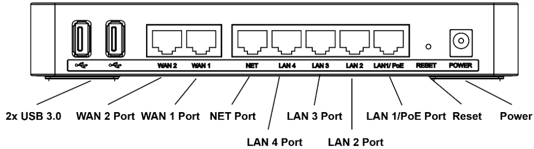
Figure 2: GWN7000 Back View
